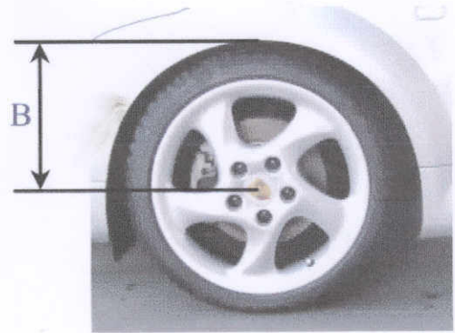
Measurement B Wheel hub center wheel arch
